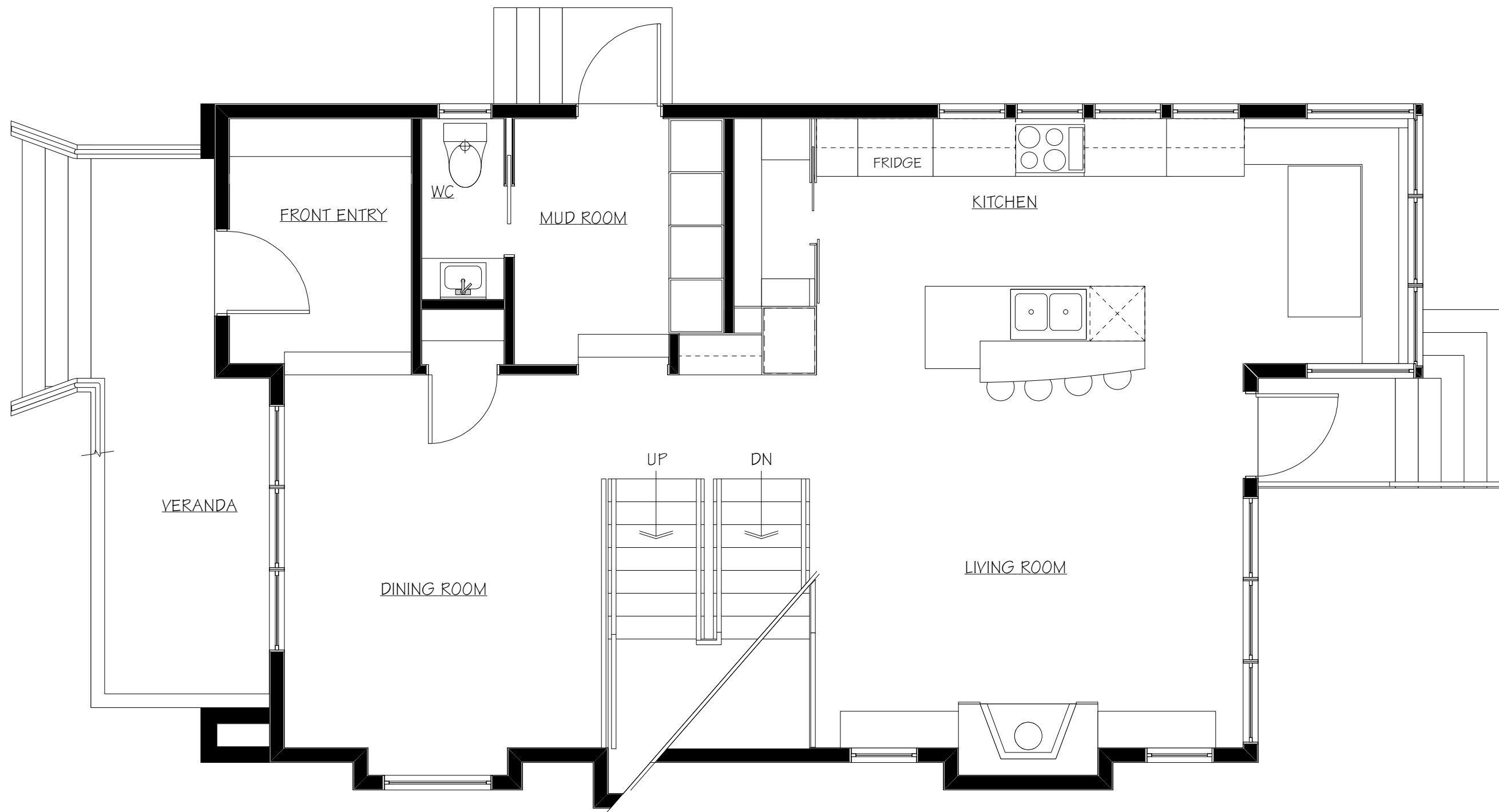
MAIN FLOOR 924 SQ. FT.
