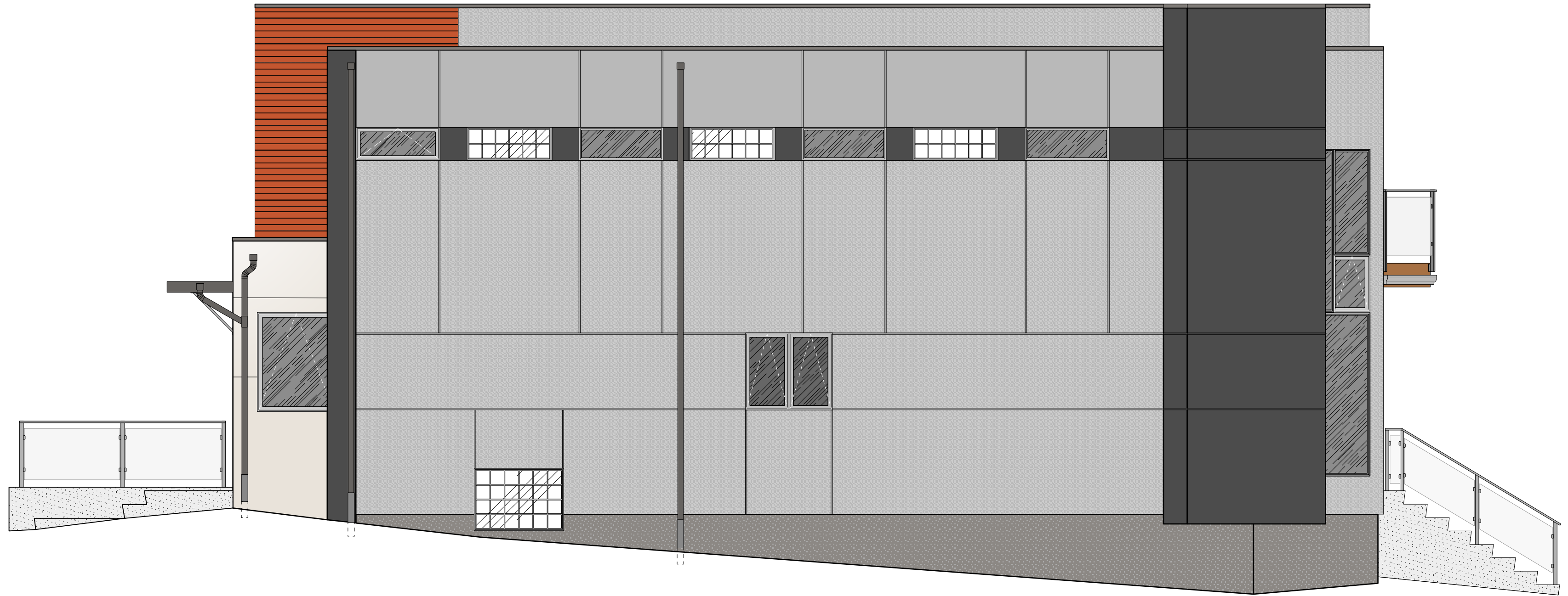
SOUTH ELEVATION
